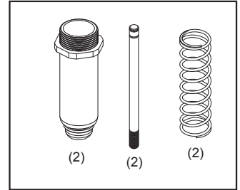
PD7734 REAR SHOCK REPAIR KIT 避震器維修組(後)
